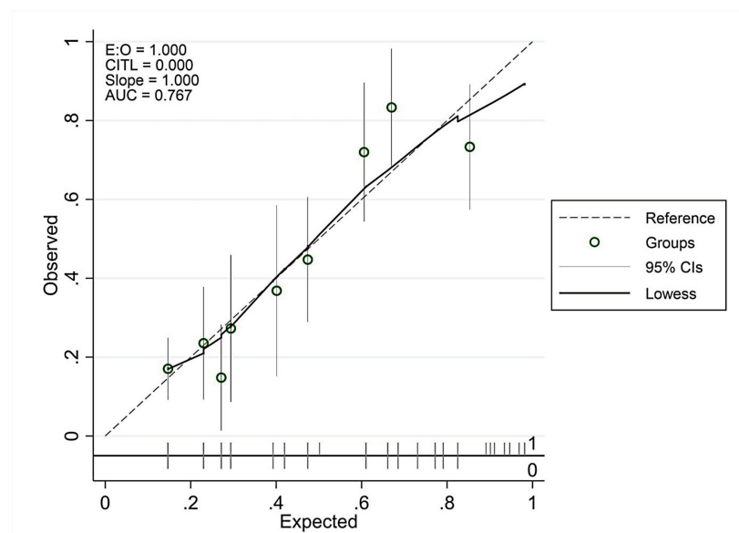
Figure 2 Pmcalplot of observed vs expected difficult laparoscopic cholecystectomy
