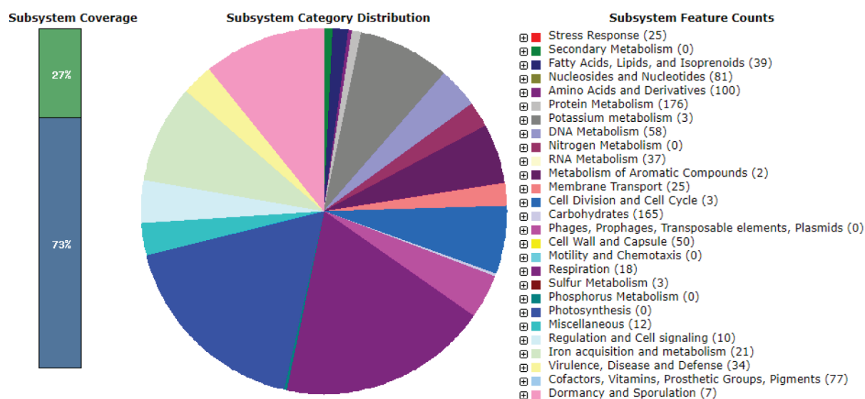
Figure 3 The subsystem coverage and distribution of functional categories within the annotated genome of the bacterial species, as analyzed using RAST
